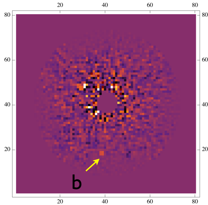
HR8799b
