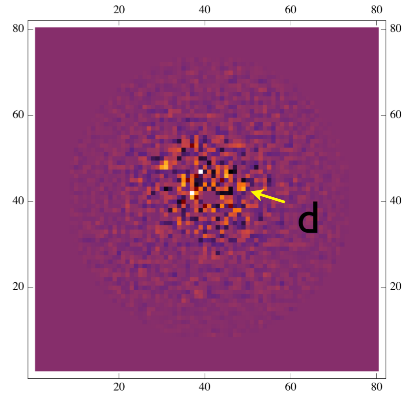
HR8799d
