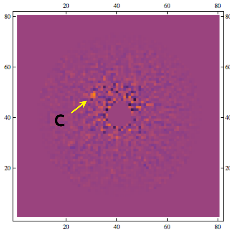
HR8799c
